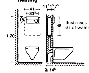
⑨ Deep-flush toilet bowl; built-in cistern
